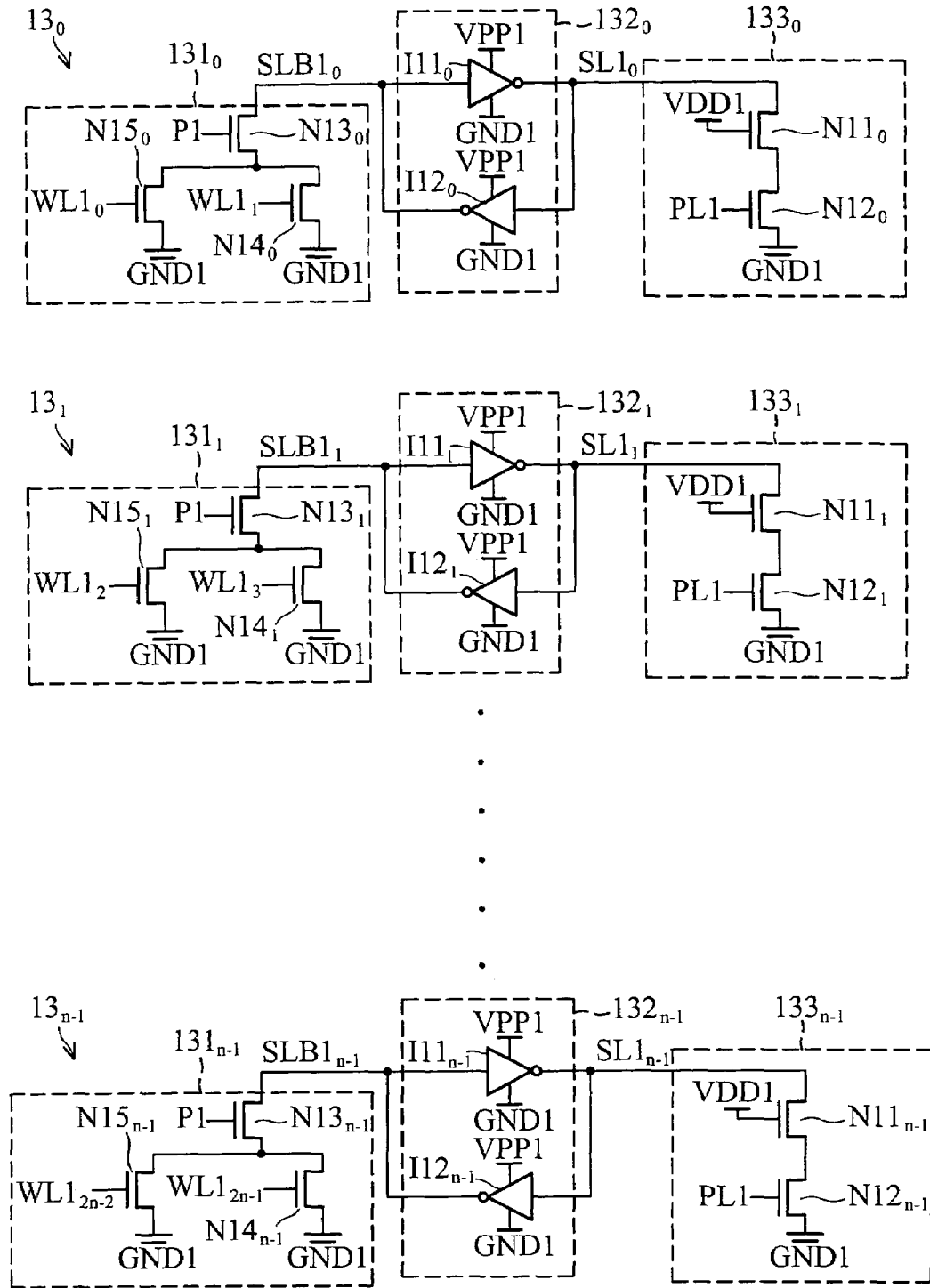
FIG. 3 (RELATED ART)
